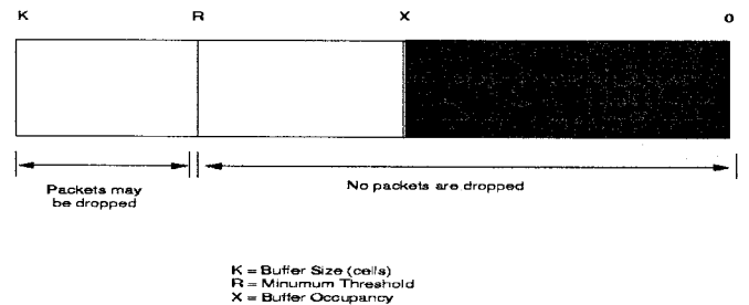
Figure 3: Selective Drop and FBA: Buffer occupancy for drop
