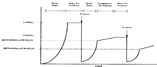
Figure 1: TCP CWND vs Time
