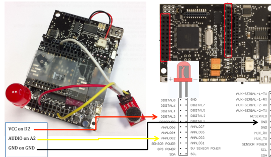
Fig. 4. Audio hardware on Libelium WaspMote
