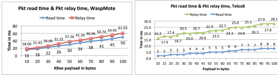
Fig. 3. Read and relaying performances: WaspMote (left) and TelosB (right)
