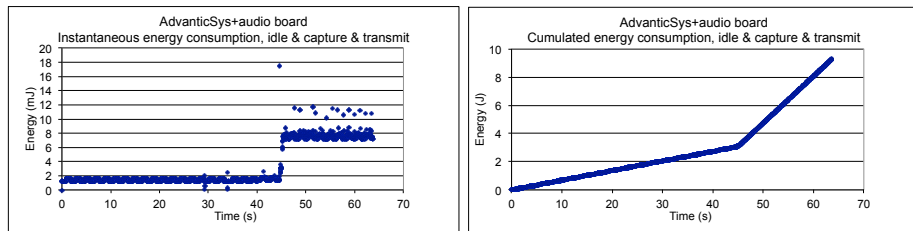
Fig. 8. Instantaneous (left) and Cumulated (right) energy consumption
